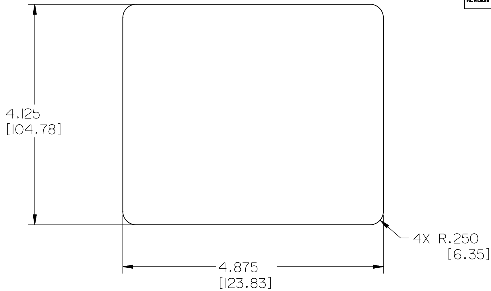
RECOMMENDED CUTOUT DETAIL
