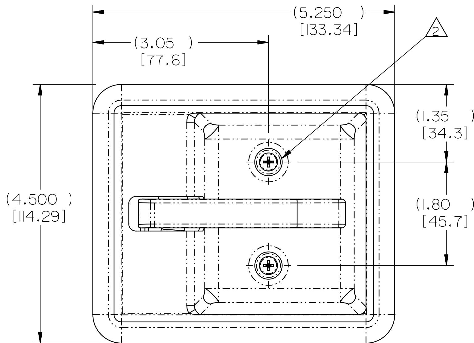
RECOMMENDED CUTOUT DETAIL
